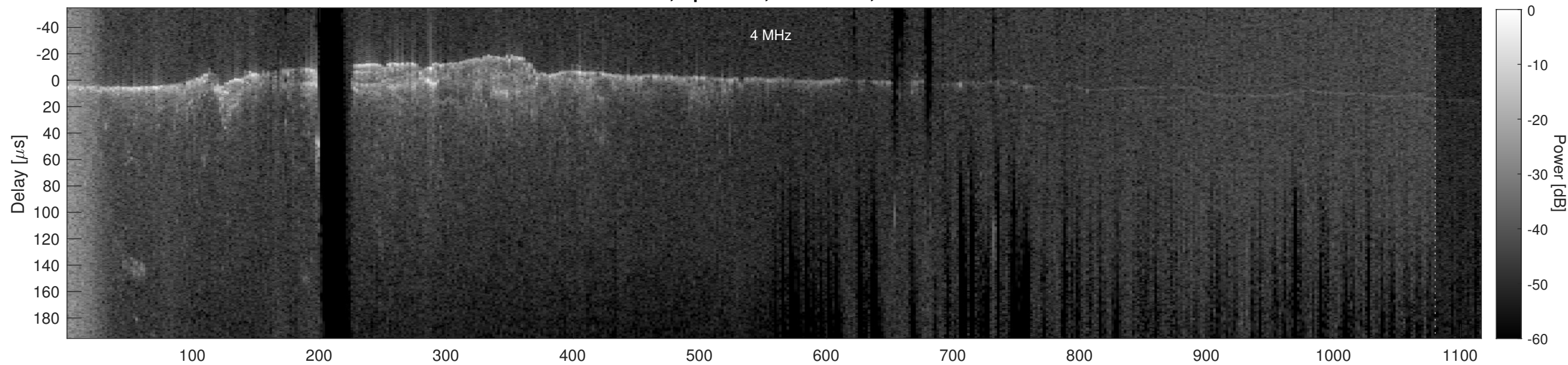
Orbit 2434, Cluttergram
