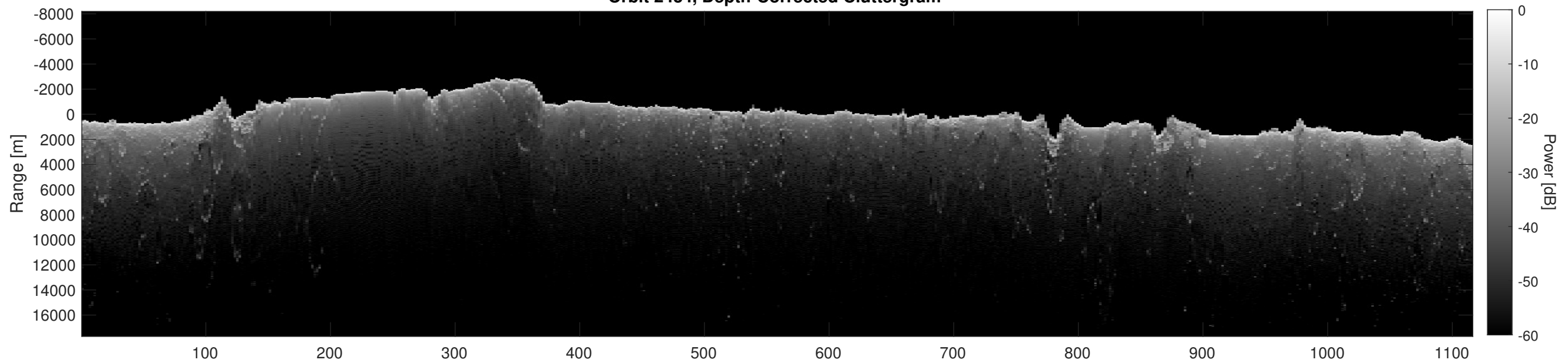
Orbit 2434, Depth-Corrected Cluttergram
