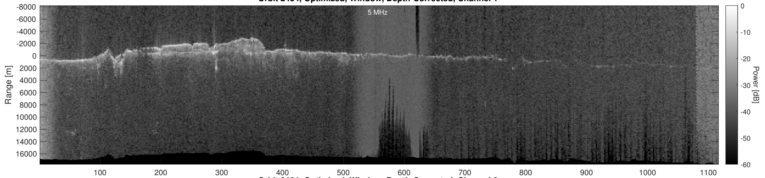
Orbit 2434, Optimized, Window, Depth-Corrected, Channel 2
