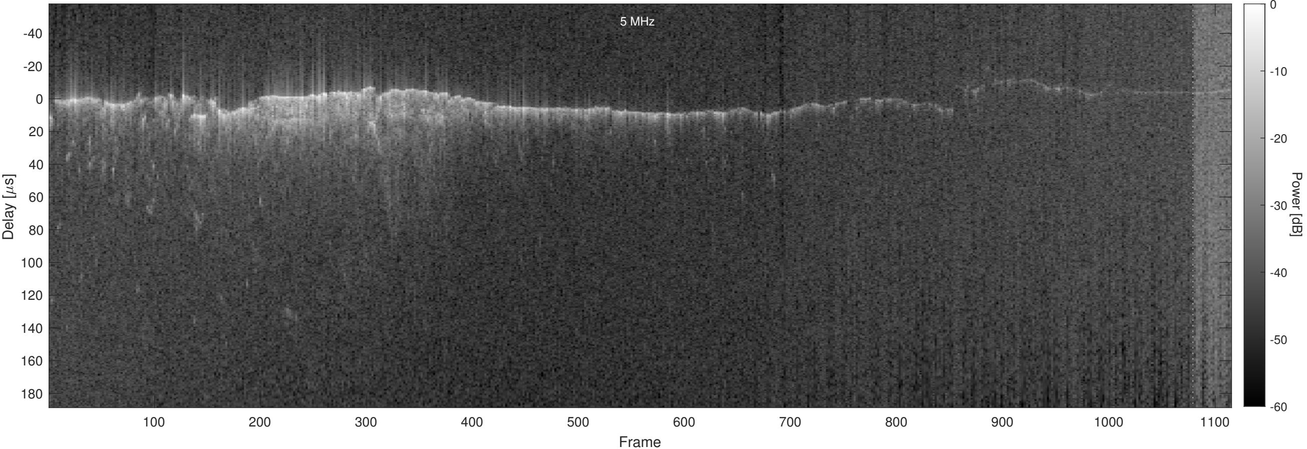
Orbit 2435, Optimized, No Window, Channel 2
