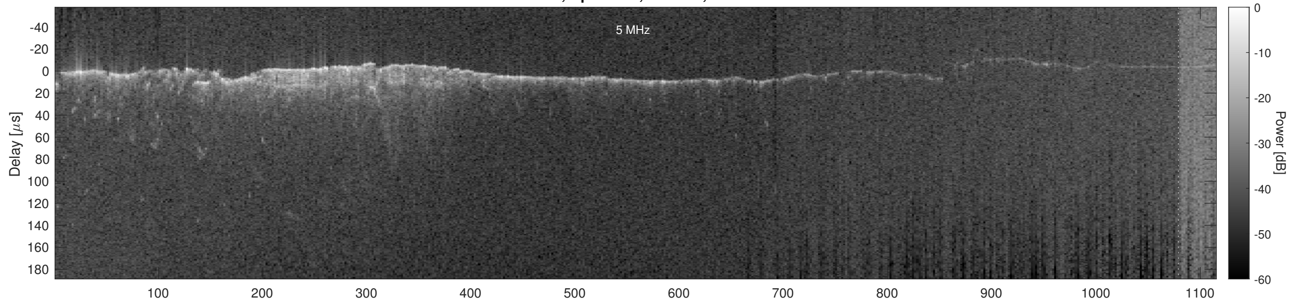
Orbit 2435, Optimized, Window, Channel 2
