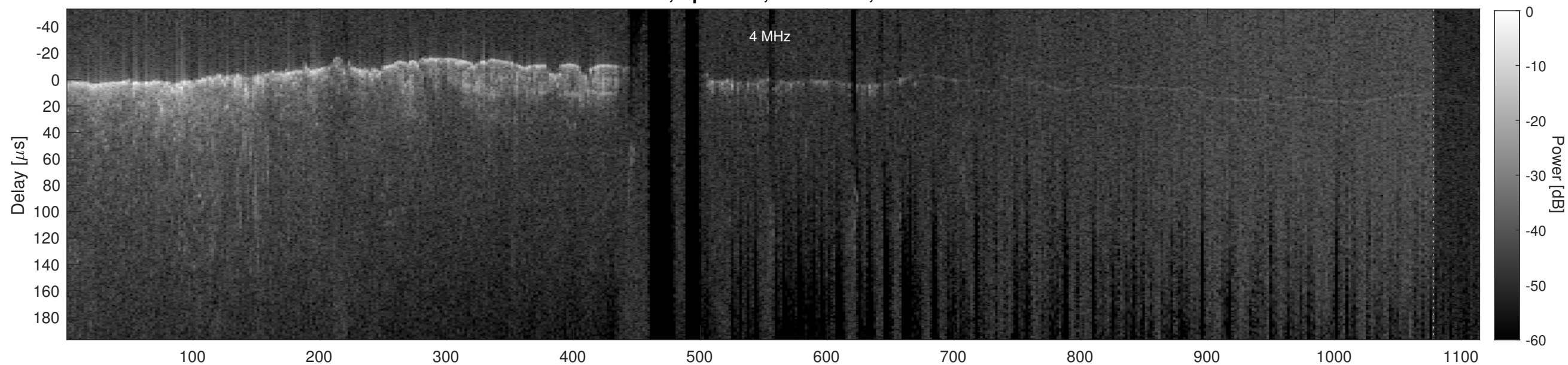
Orbit 2436, Cluttergram
