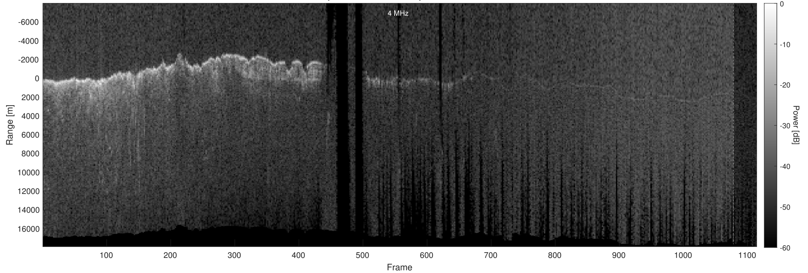
Orbit 2436, Optimized, Window, Depth-Corrected, Channel 2
