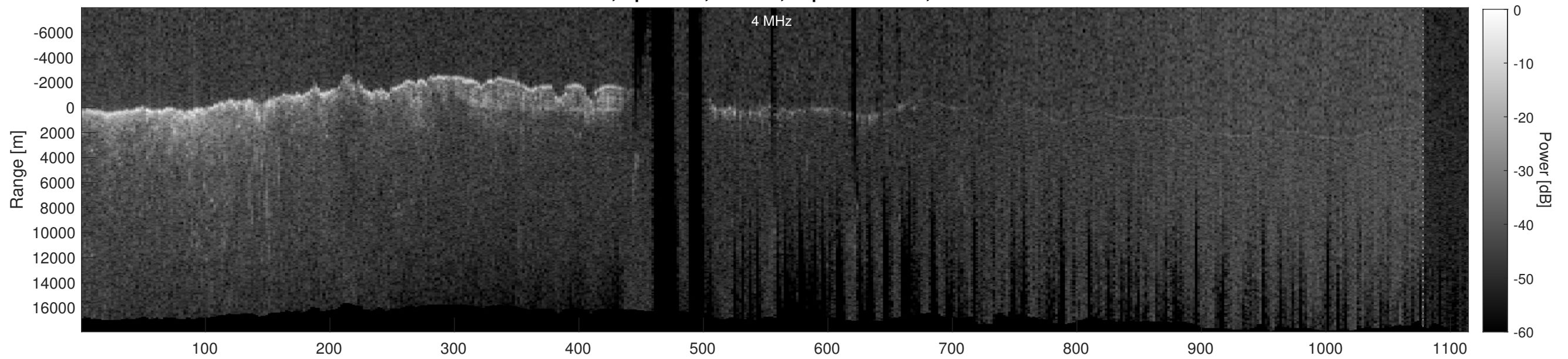
Orbit 2436, Depth-Corrected Cluttergram
