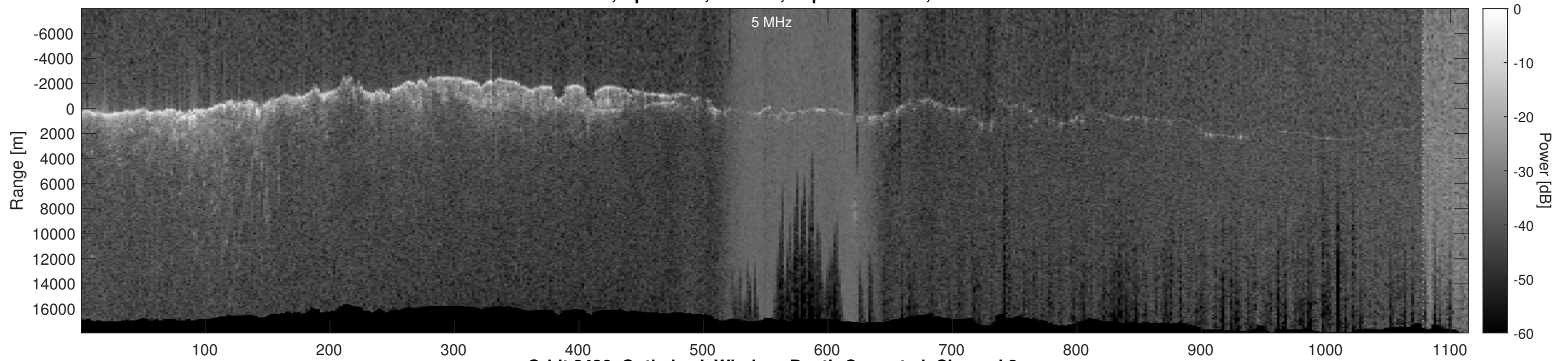
Orbit 2436, Optimized, Window, Depth-Corrected, Channel 2
