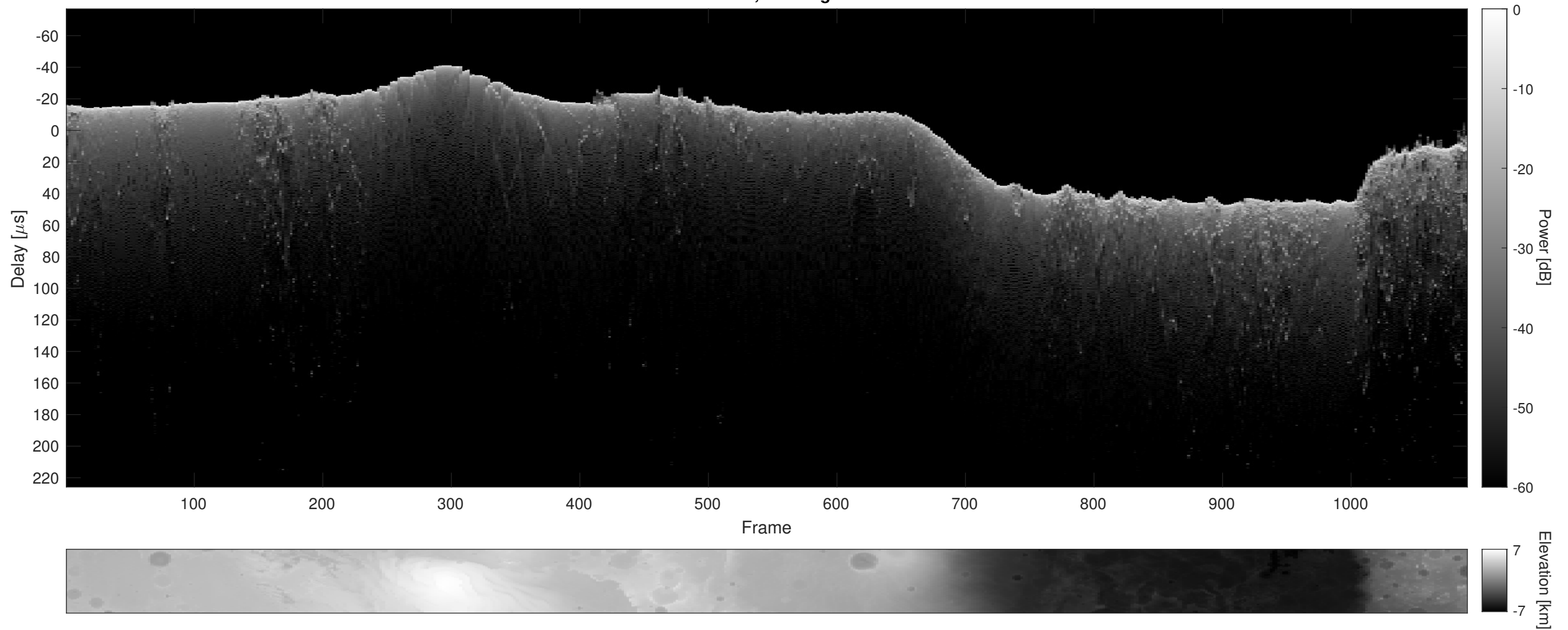
Orbit 2437, Cluttergram
