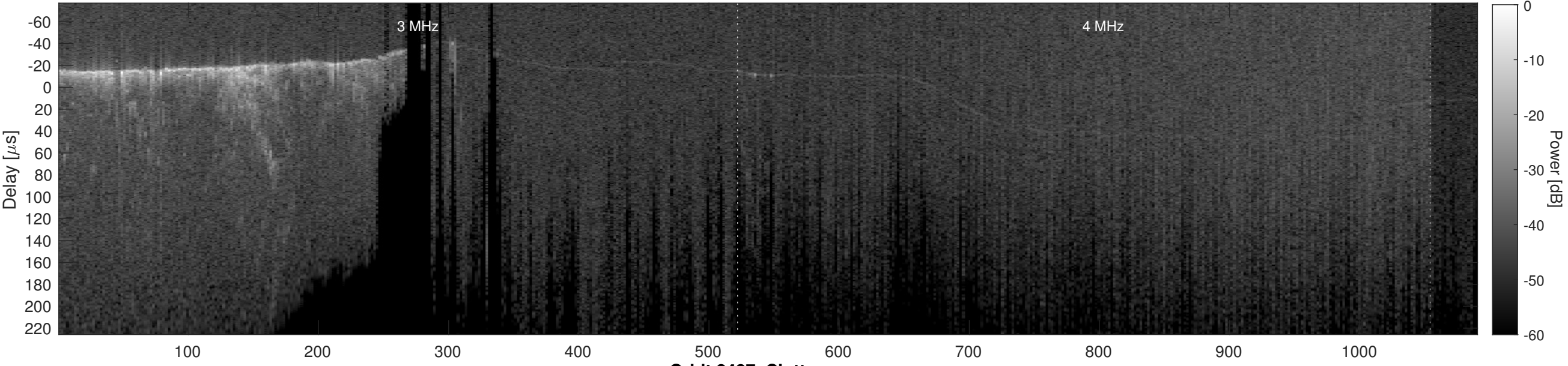
Orbit 2437, Cluttergram
