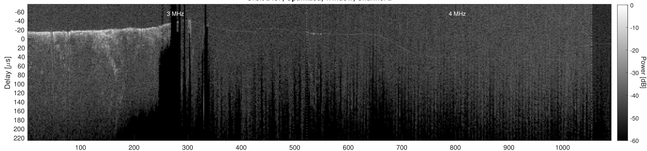
Orbit 2437, Cluttergram
