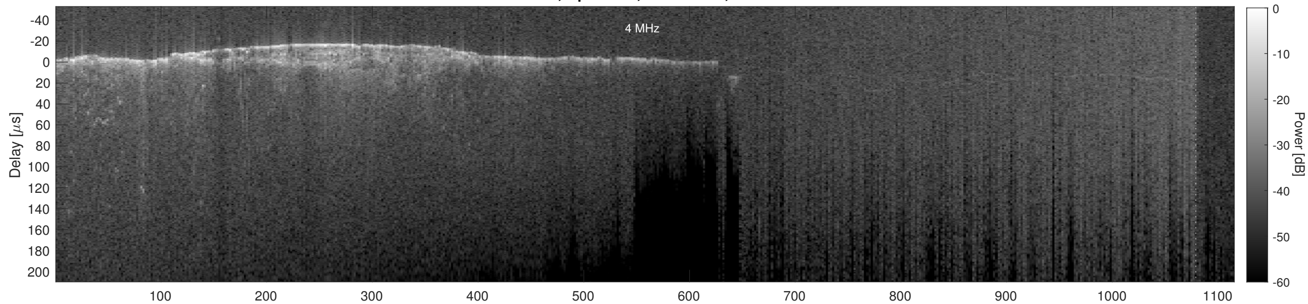
Orbit 2438, Cluttergram
