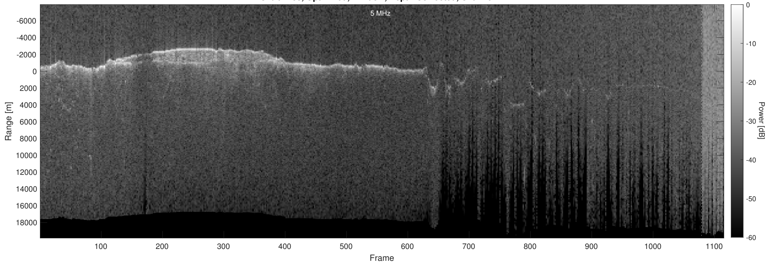
Orbit 2438, Optimized, Window, Depth-Corrected, Channel 2
