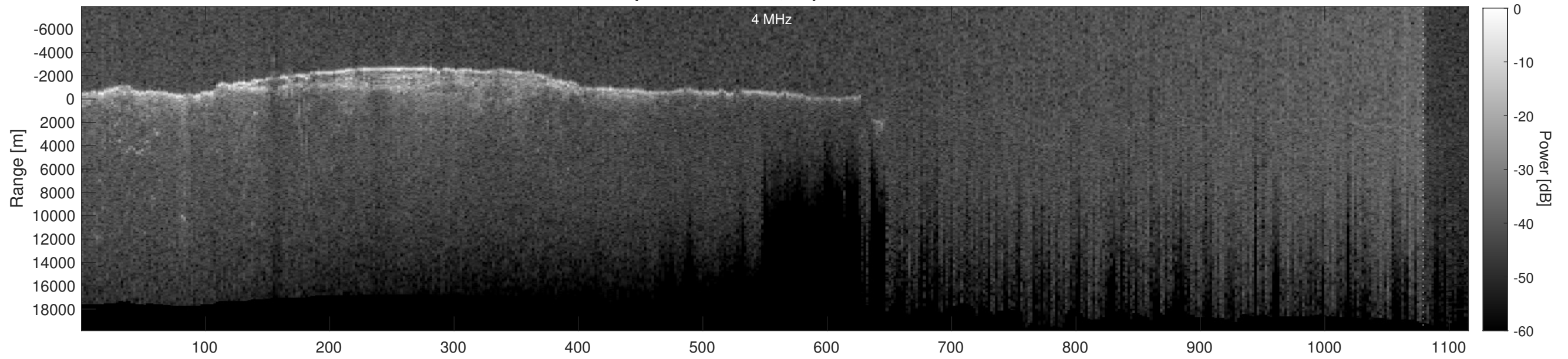
Orbit 2438, Depth-Corrected Cluttergram
