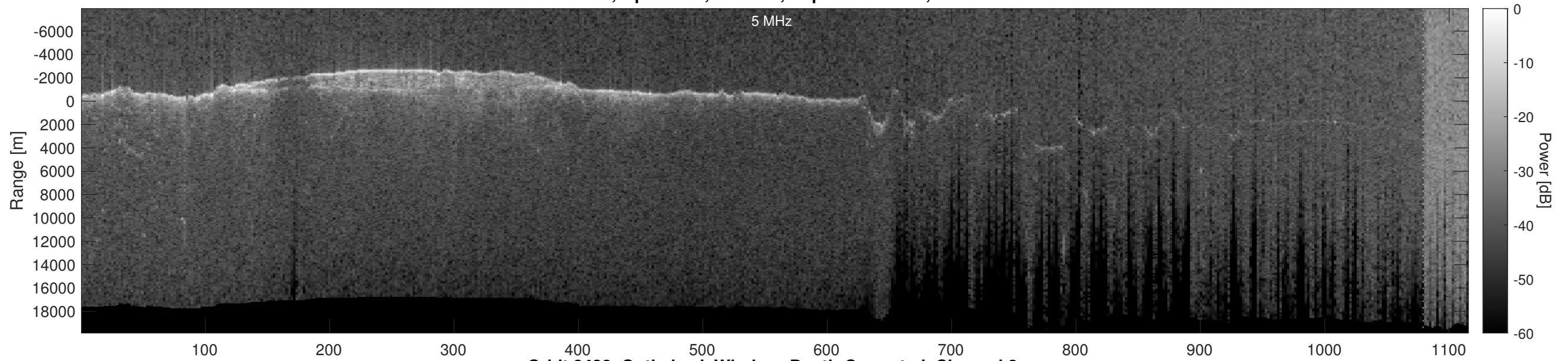
Orbit 2438, Optimized, Window, Depth-Corrected, Channel 2
