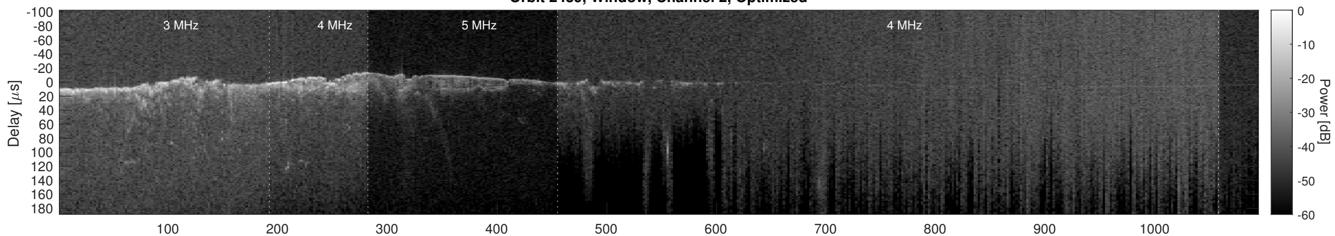
Orbit 2439, Cluttergram
