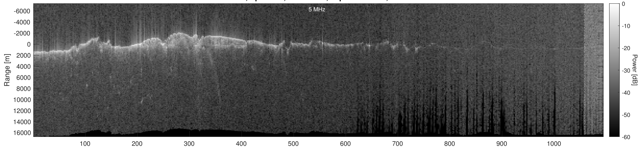
Orbit 2439, Optimized, No Window, Depth-Corrected, Channel 2
