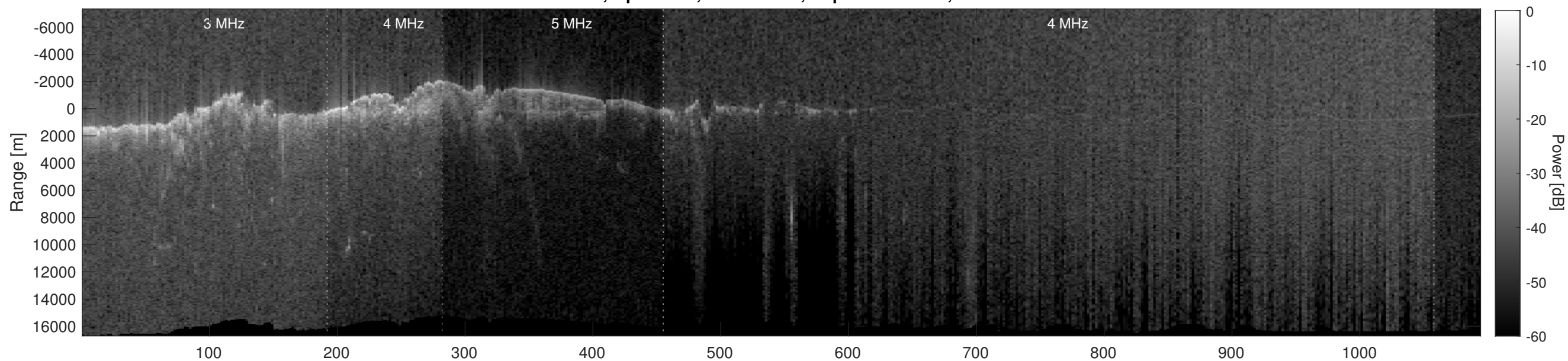
Orbit 2439, Depth-Corrected Cluttergram
