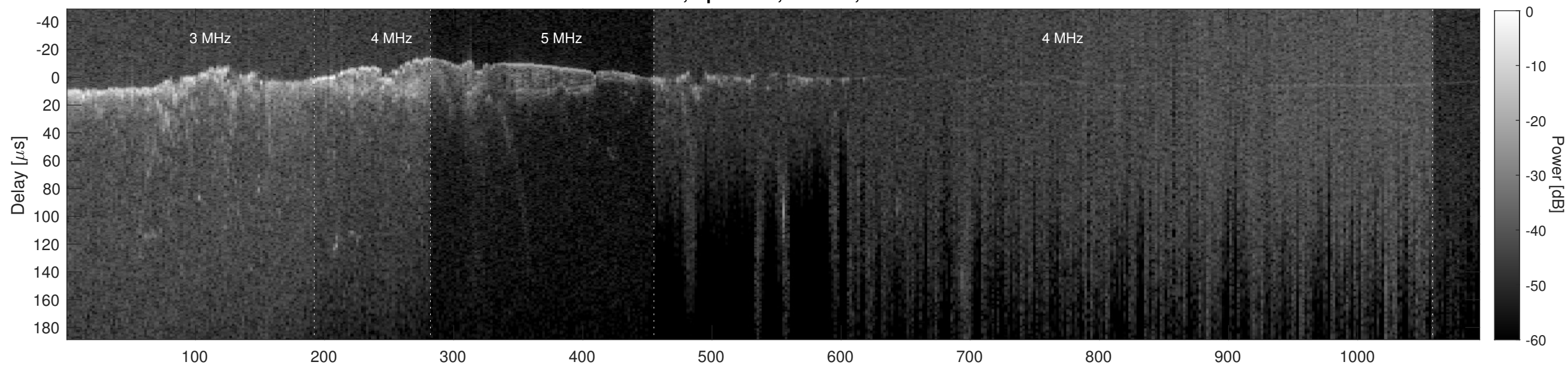
Orbit 2439, Cluttergram
