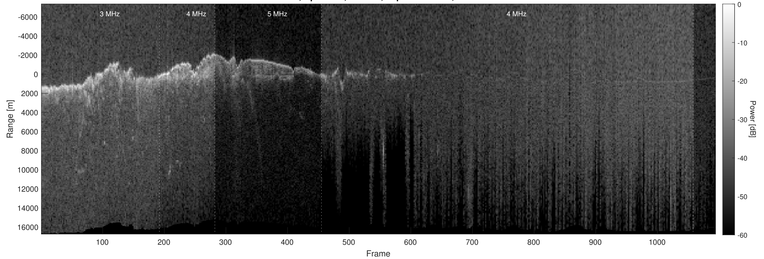
Orbit 2439, Optimized, Window, Depth-Corrected, Channel 2
