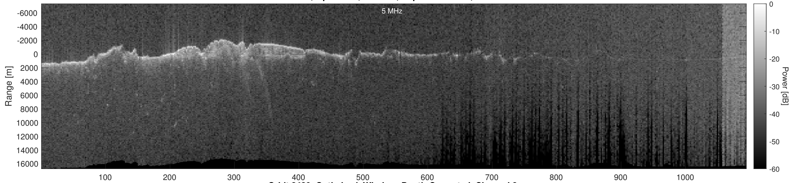
Orbit 2439, Optimized, Window, Depth-Corrected, Channel 2
