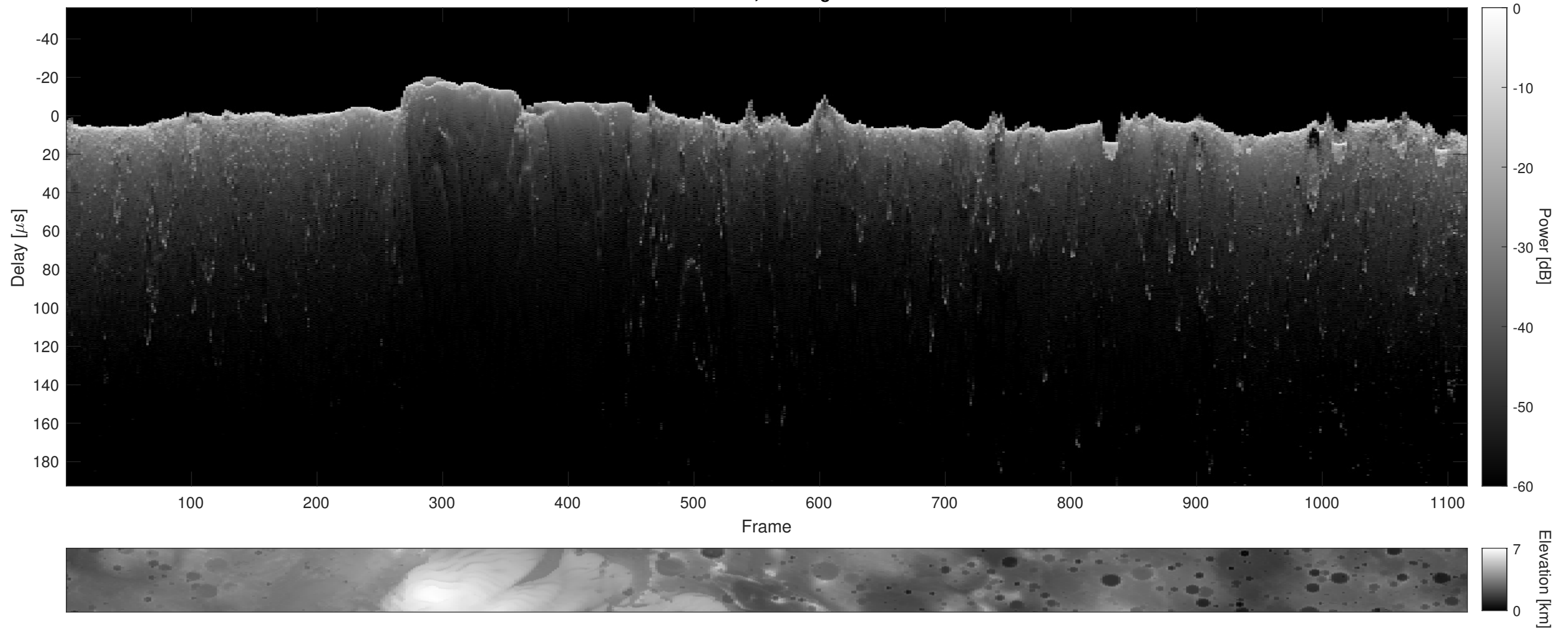
Orbit 2440, Cluttergram
