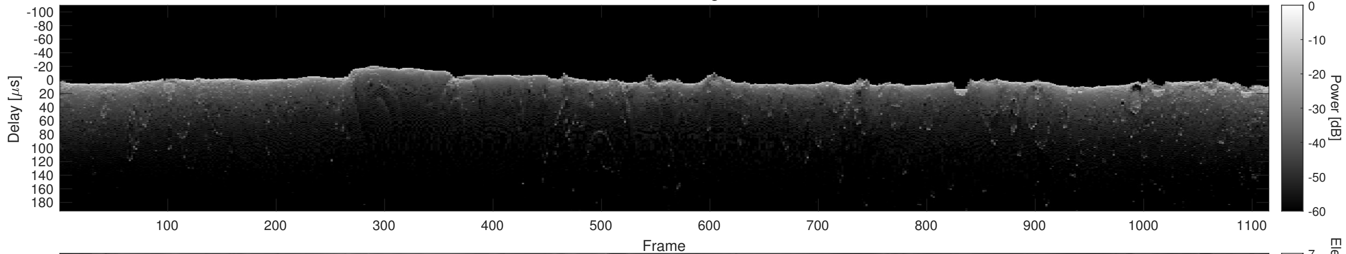
Orbit 2440, Cluttergram
