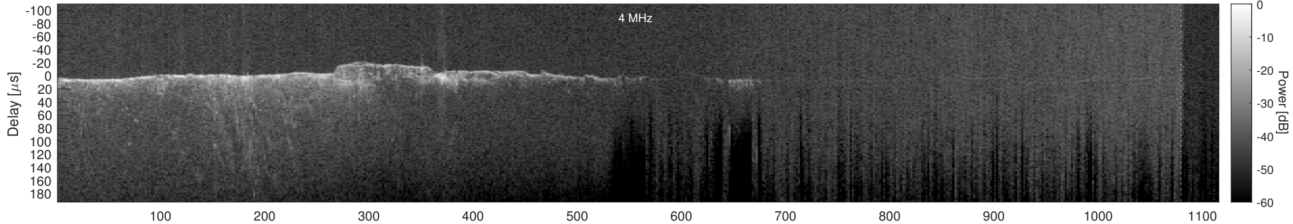
Orbit 2440, Cluttergram
