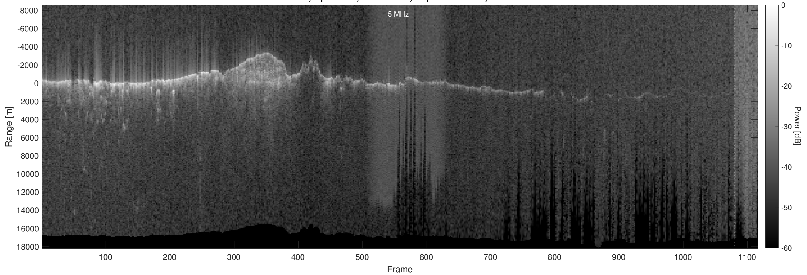
Orbit 2441, Optimized, No Window, Depth-Corrected, Channel 2
