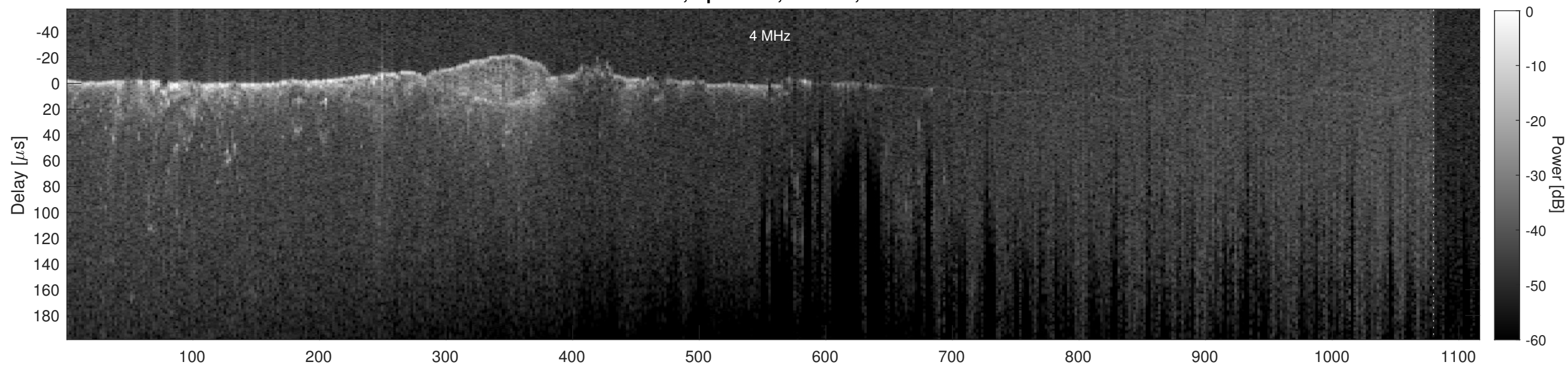
Orbit 2441, Cluttergram
