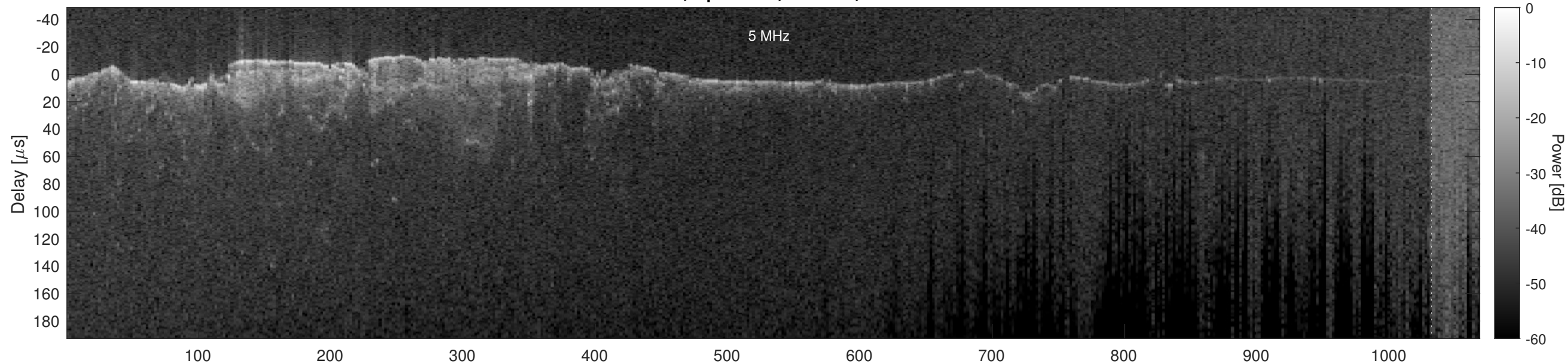
Orbit 2442, Optimized, Window, Channel 2
