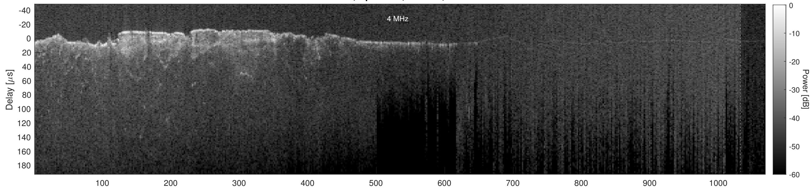
Orbit 2442, Cluttergram
