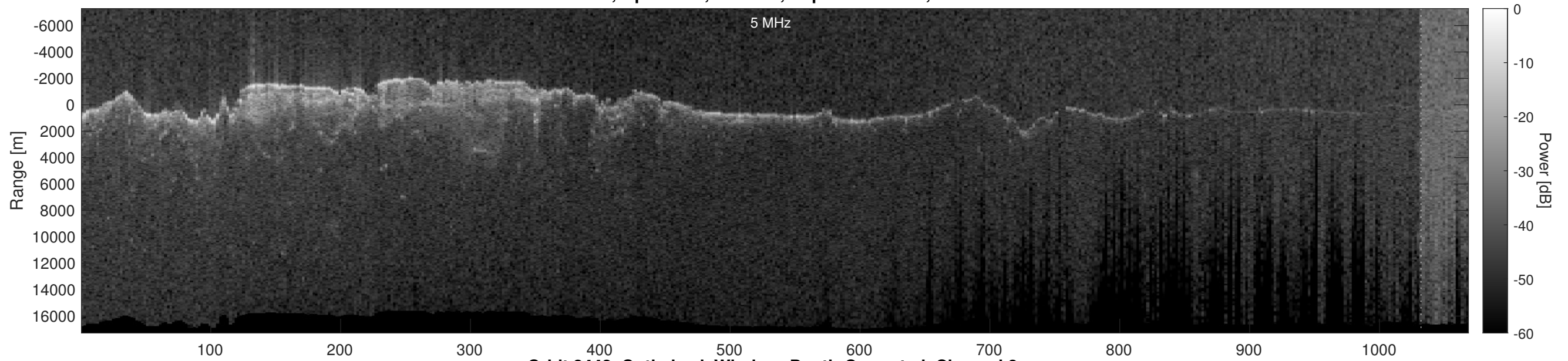
Orbit 2442, Optimized, Window, Depth-Corrected, Channel 2
