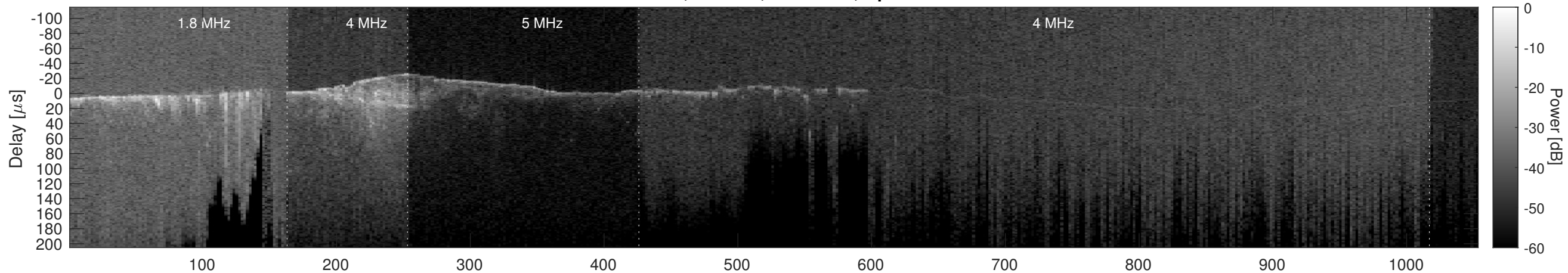
Orbit 2444, Cluttergram
