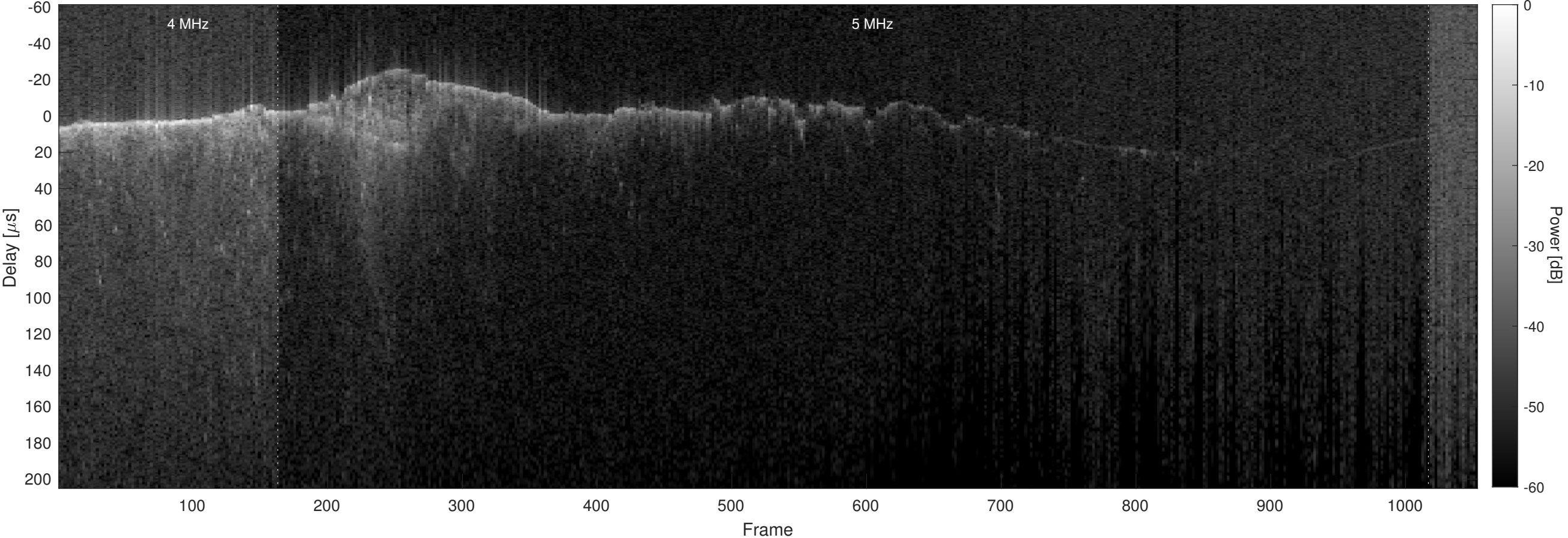
Orbit 2444, Optimized, No Window, Channel 2
