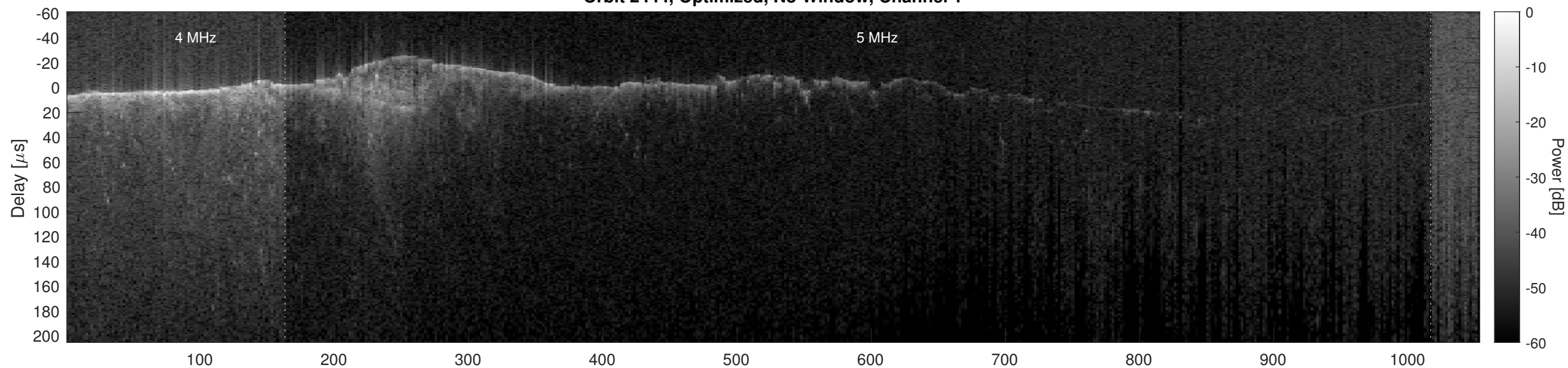
Orbit 2444, Optimized, No Window, Channel 2
