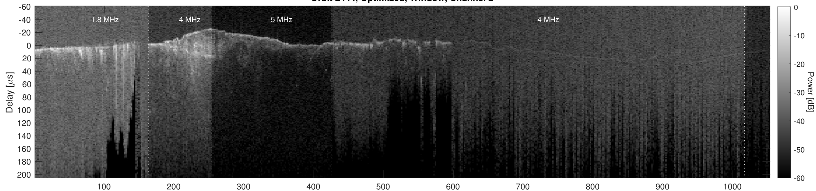
Orbit 2444, Cluttergram
