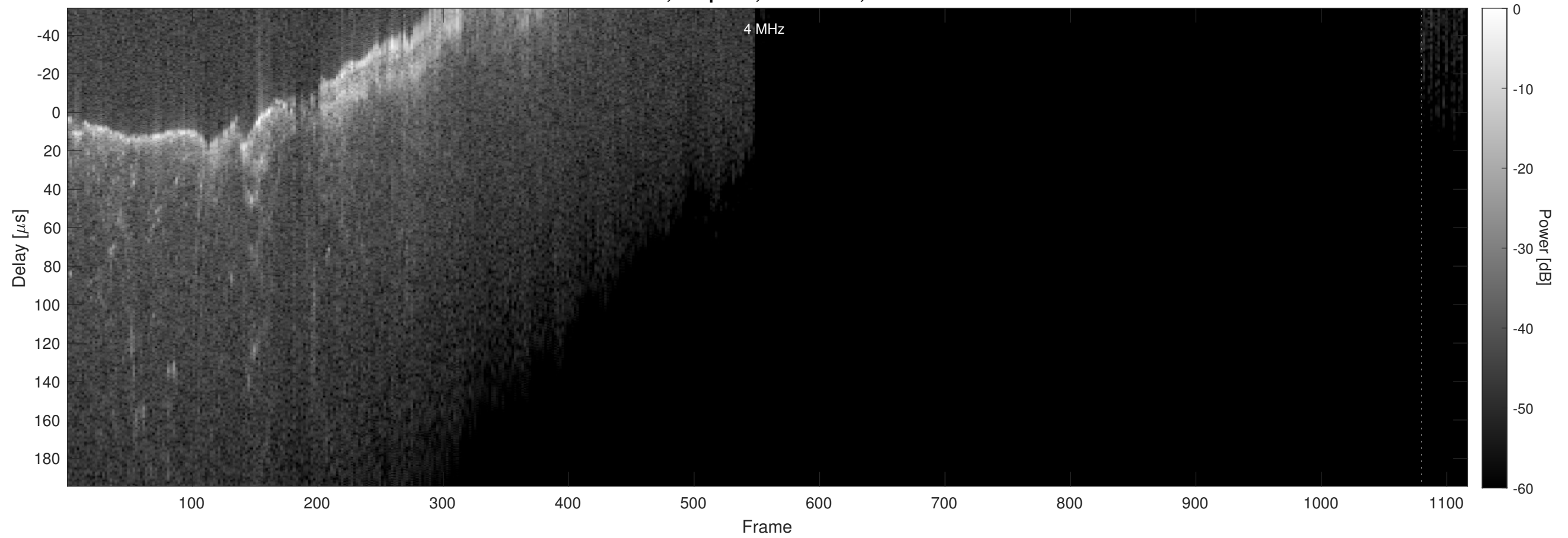
Orbit 2445, Chapman, No Window, Channel 2
