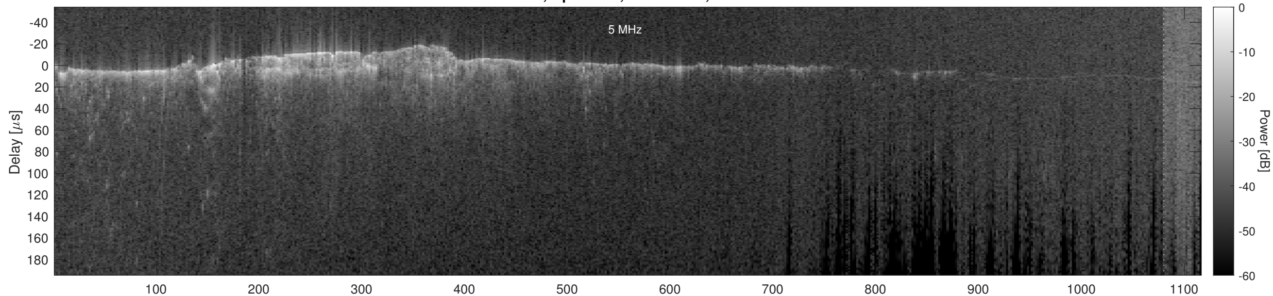
Orbit 2445, Optimized, No Window, Channel 2
