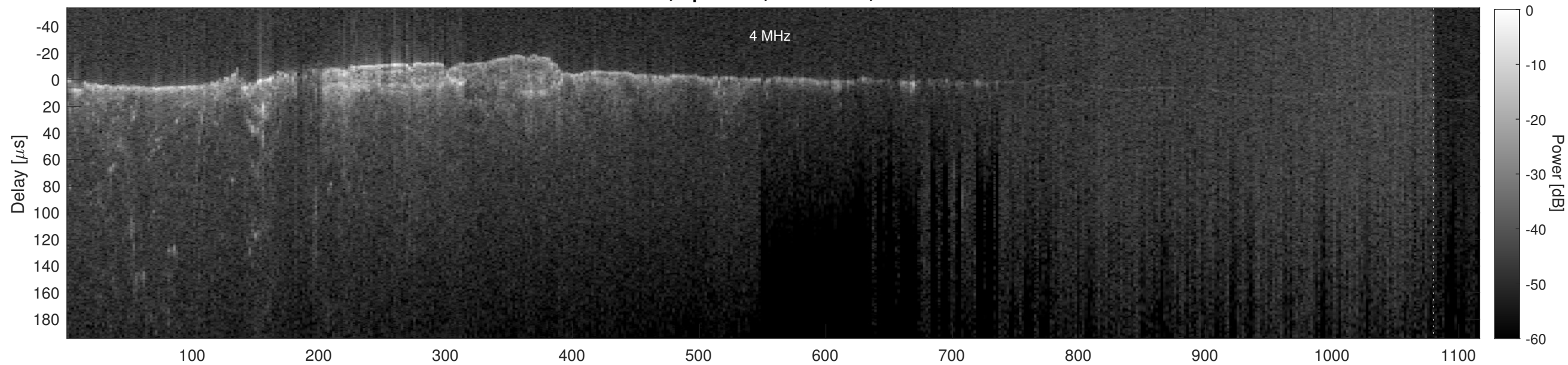
Orbit 2445, Cluttergram
