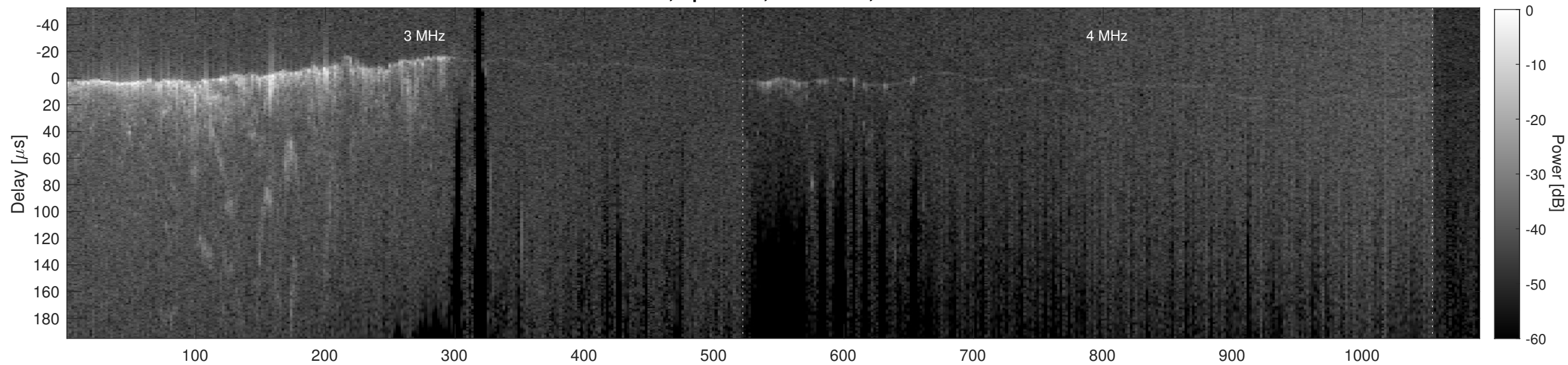
Orbit 2447, Cluttergram
