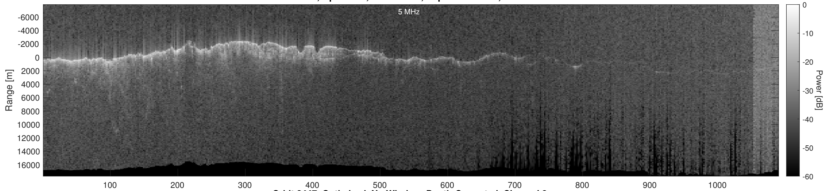
Orbit 2447, Optimized, No Window, Depth-Corrected, Channel 2
