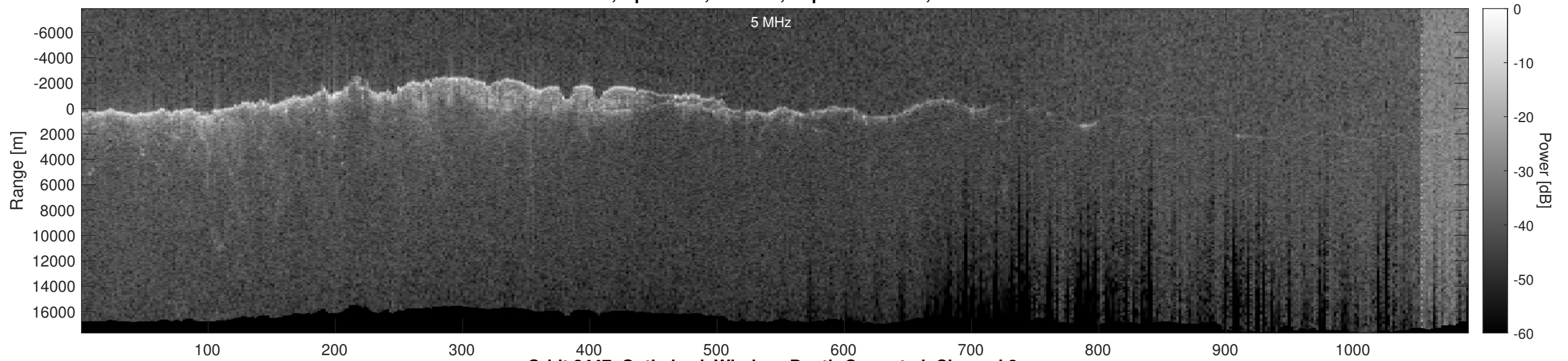
Orbit 2447, Optimized, Window, Depth-Corrected, Channel 2
