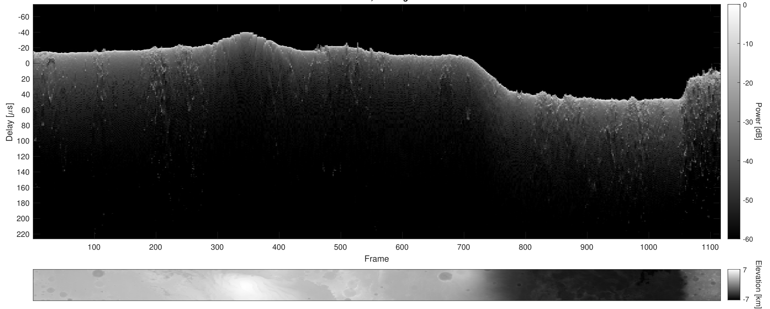
Orbit 2448, Cluttergram
