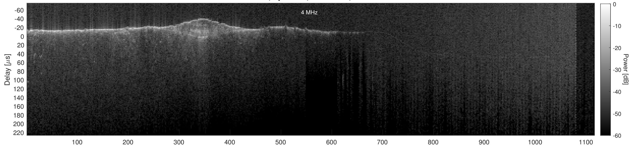
Orbit 2448, Cluttergram
