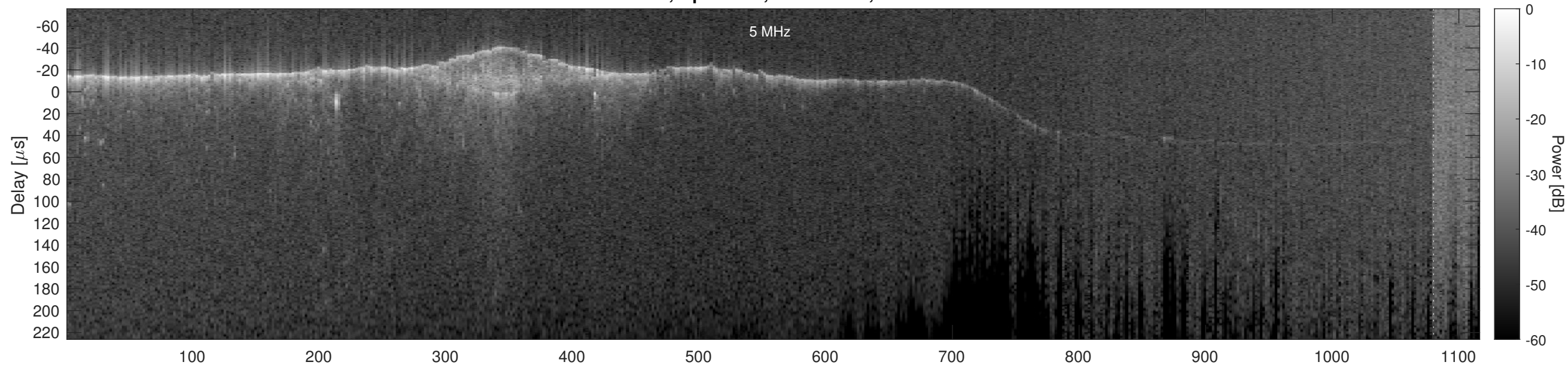
Orbit 2448, Optimized, No Window, Channel 2
