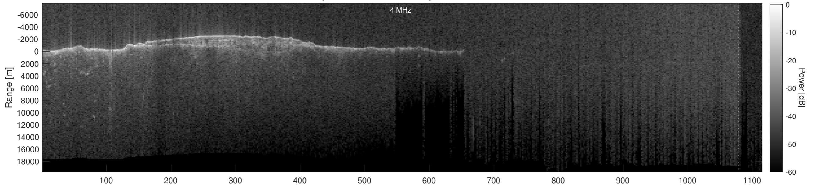
Orbit 2449, Depth-Corrected Cluttergram
