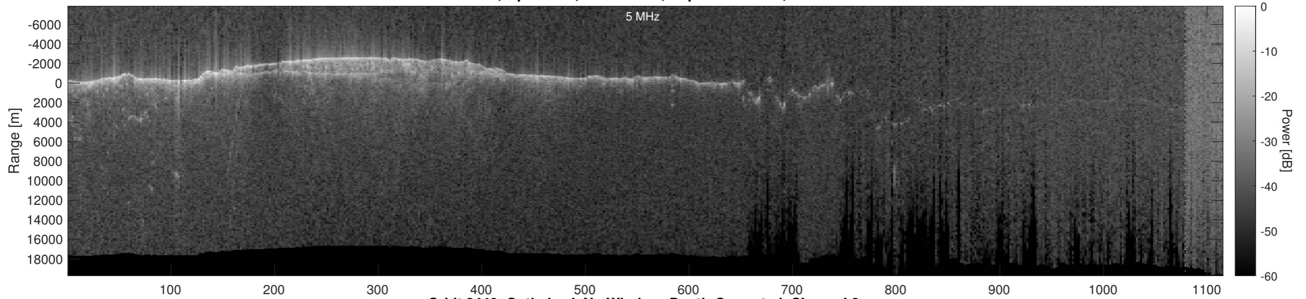
Orbit 2449, Optimized, No Window, Depth-Corrected, Channel 2
