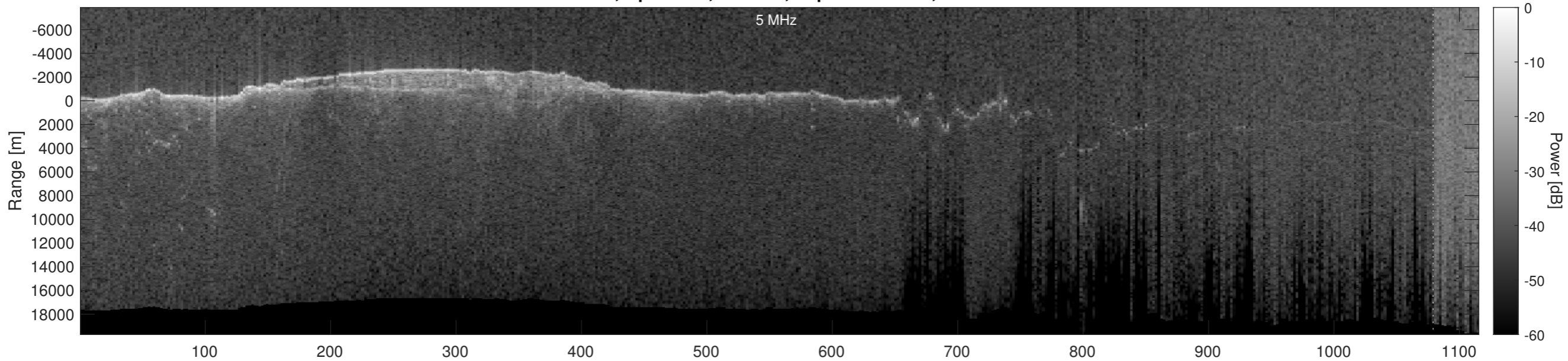
Orbit 2449, Optimized, Window, Depth-Corrected, Channel 2
