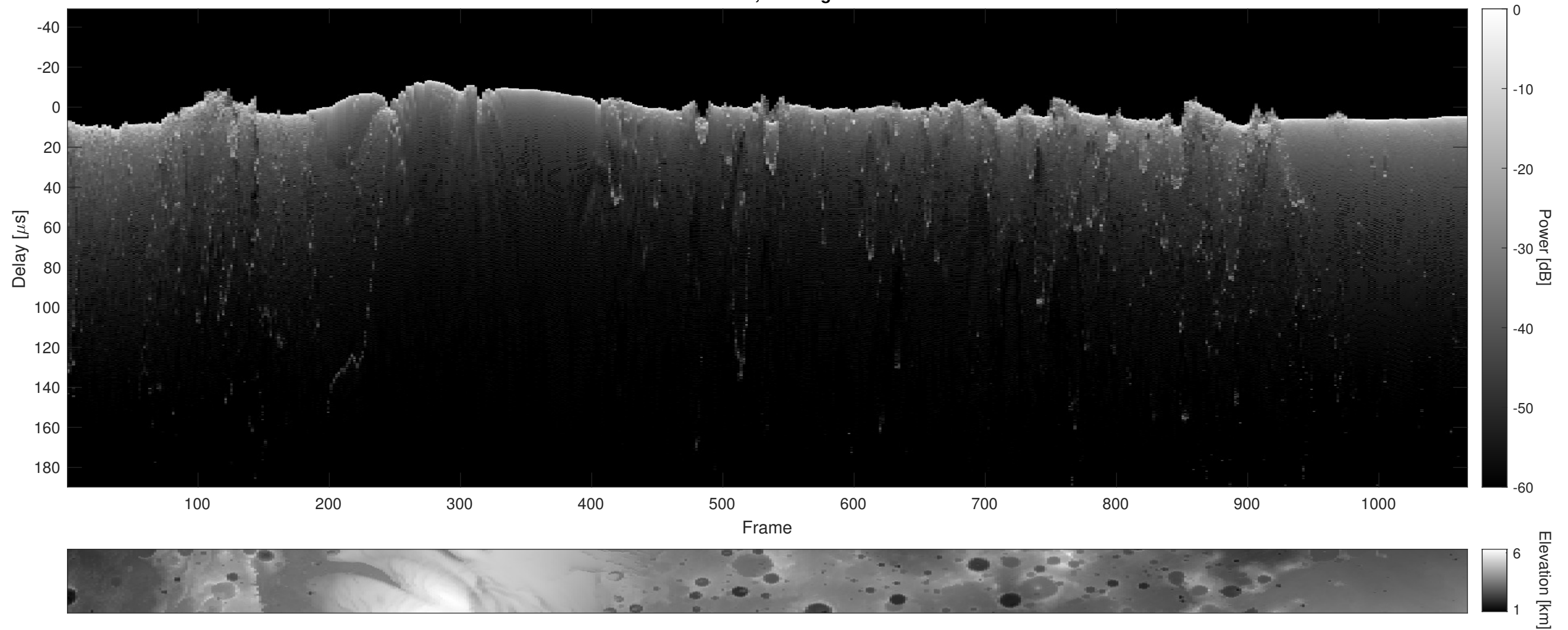
Orbit 2450, Cluttergram
