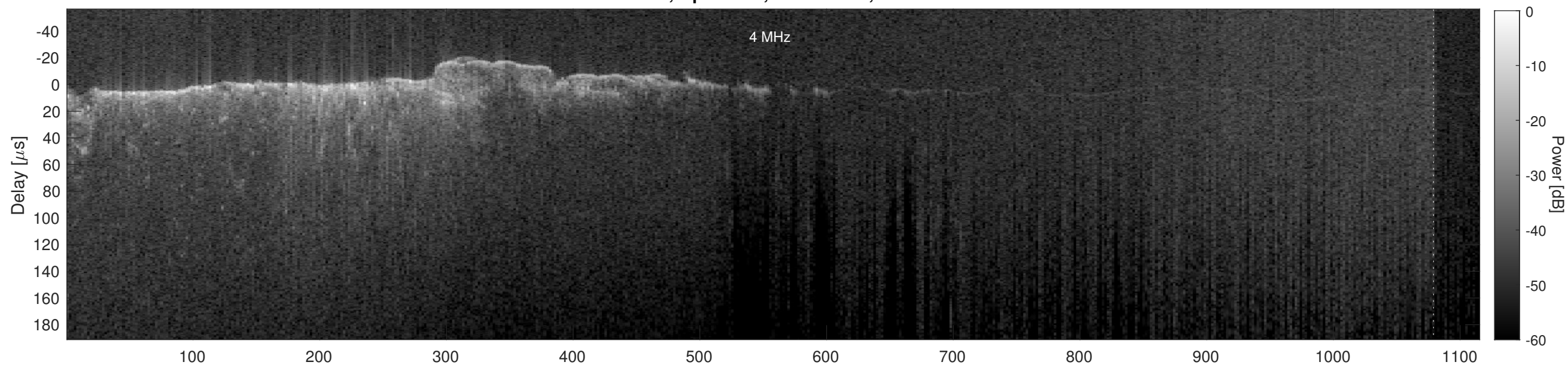
Orbit 2451, Cluttergram
