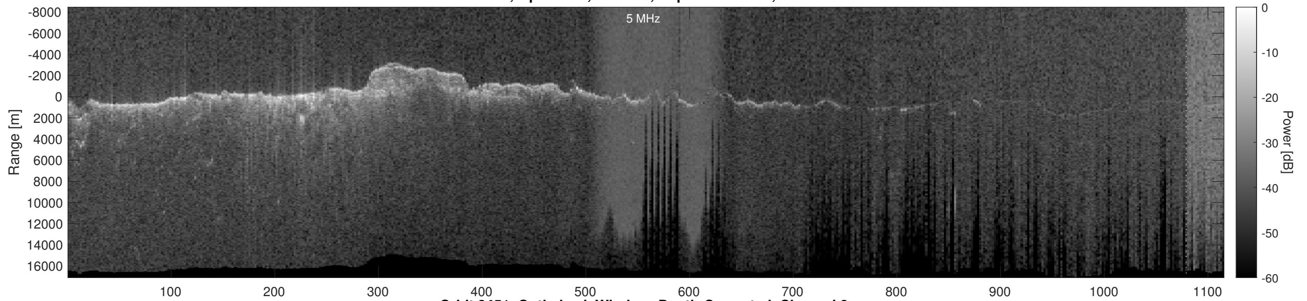
Orbit 2451, Optimized, Window, Depth-Corrected, Channel 2
