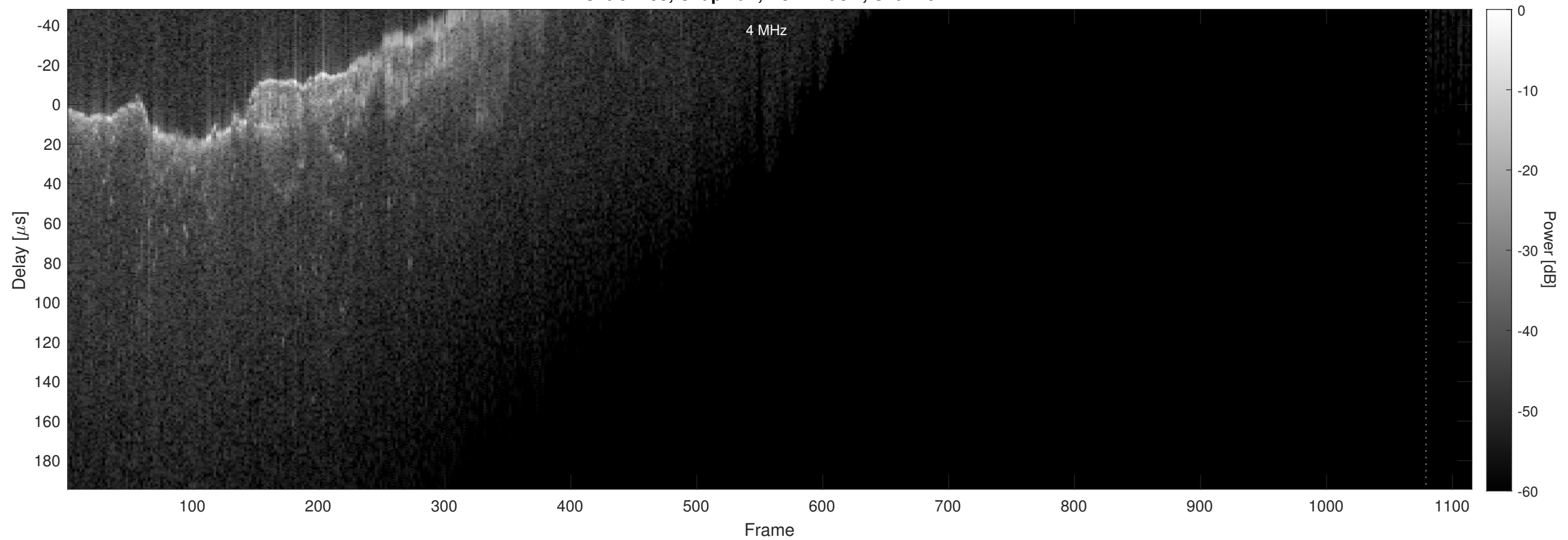
Orbit 2453, Chapman, No Window, Channel 2
