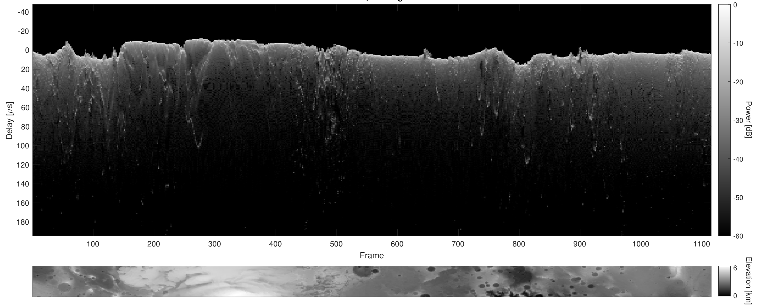
Orbit 2453, Cluttergram
