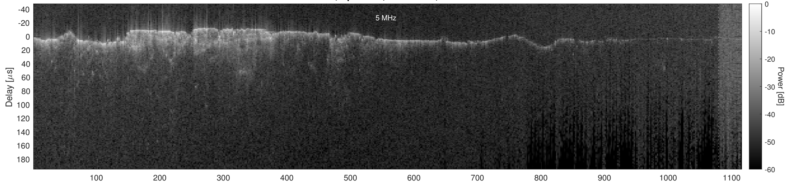
Orbit 2453, Optimized, No Window, Channel 2
