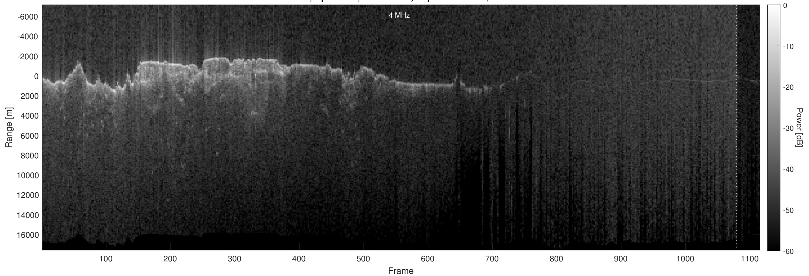
Orbit 2453, Optimized, No Window, Depth-Corrected, Channel 2
