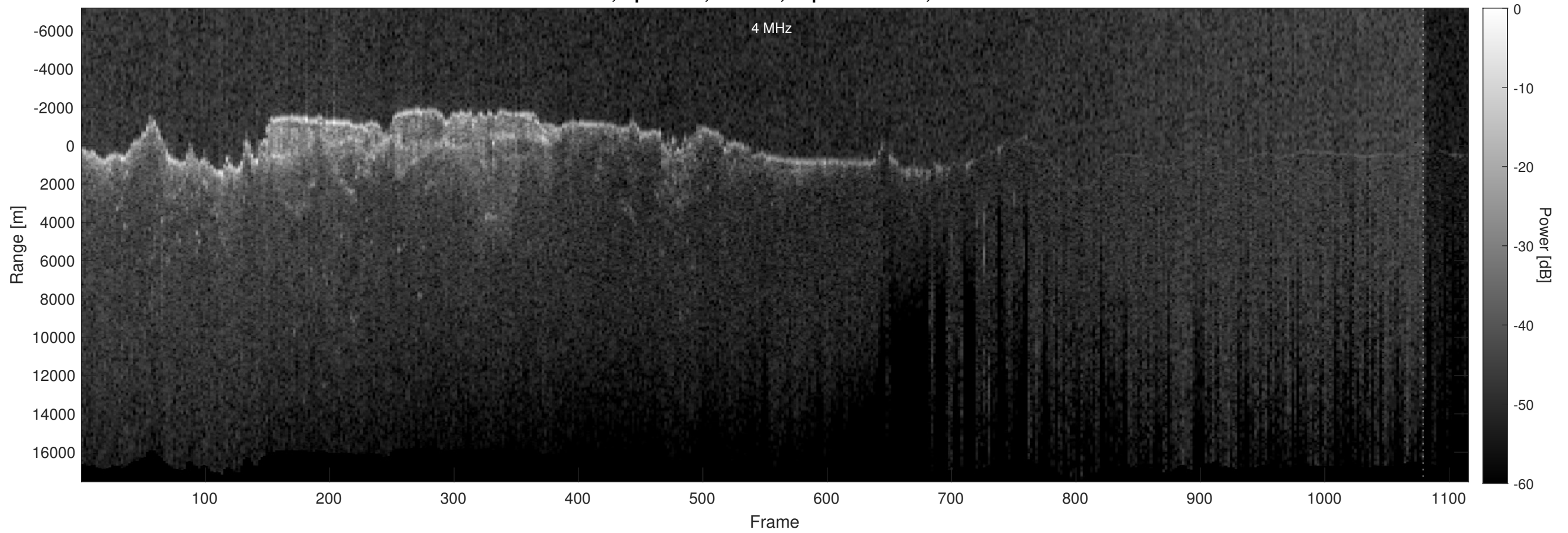
Orbit 2453, Optimized, Window, Depth-Corrected, Channel 2
