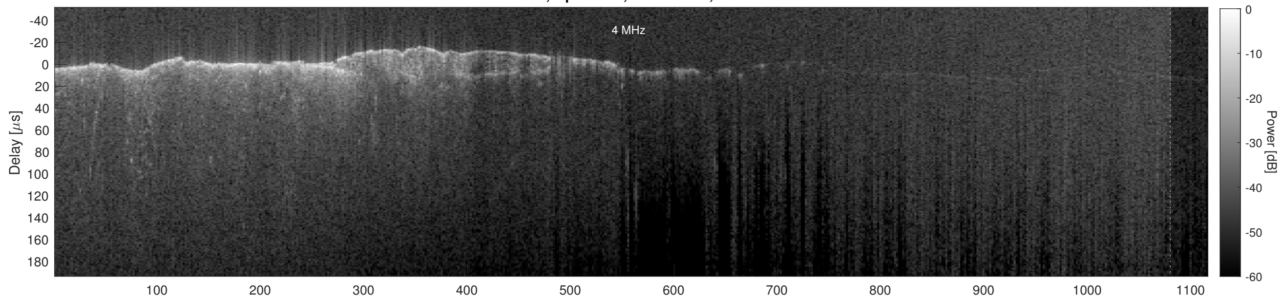
Orbit 2454, Cluttergram
