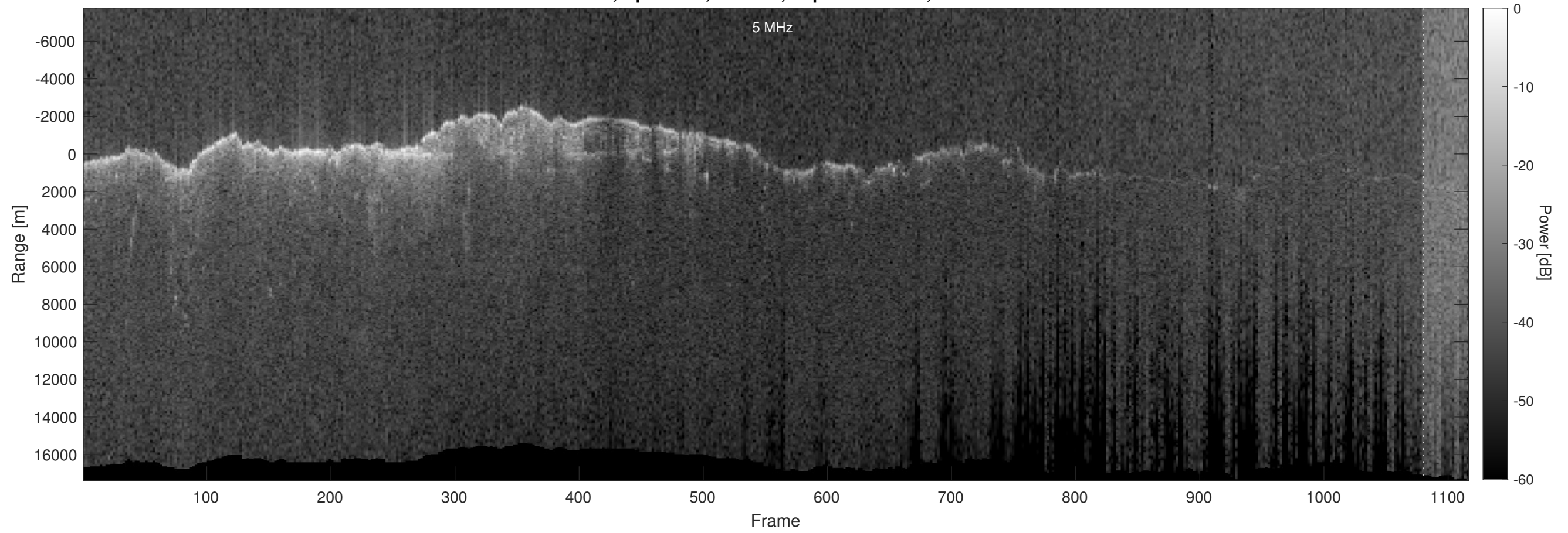
Orbit 2454, Optimized, Window, Depth-Corrected, Channel 2
