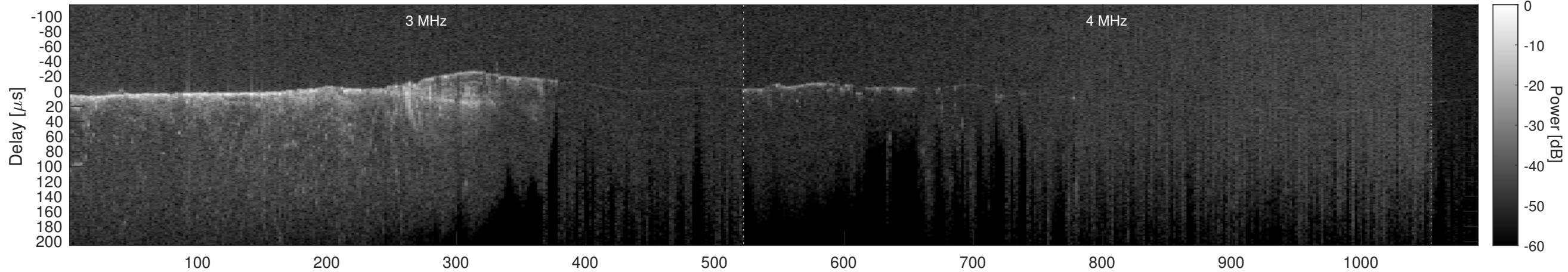
Orbit 2455, Cluttergram
