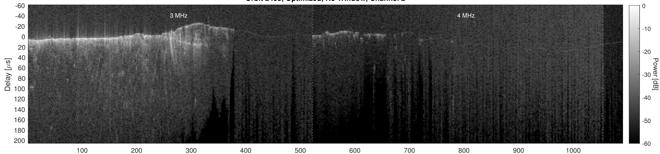
Orbit 2455, Cluttergram
