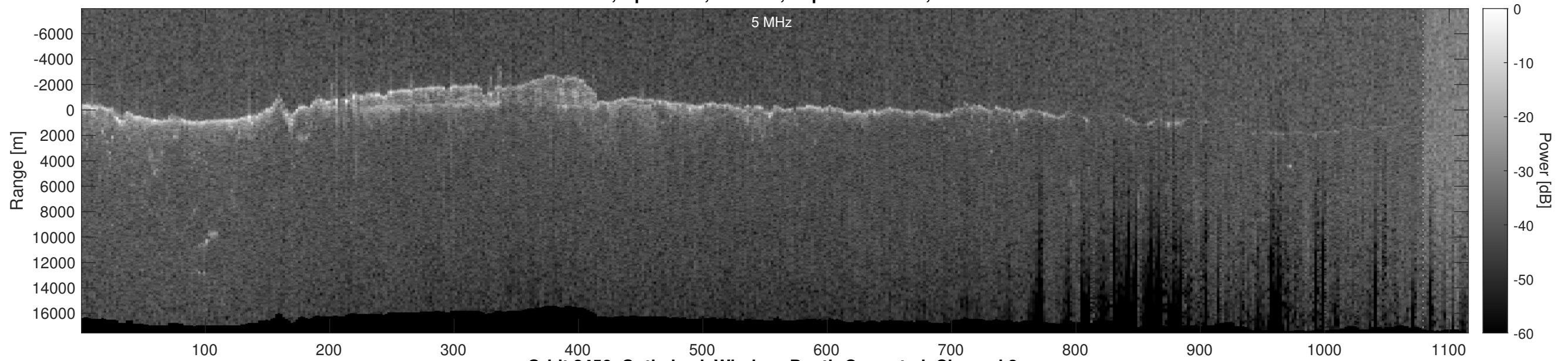
Orbit 2456, Optimized, Window, Depth-Corrected, Channel 2
