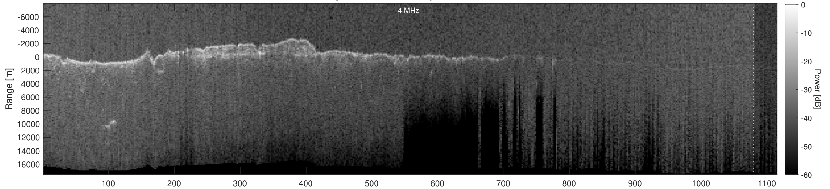
Orbit 2456, Depth-Corrected Cluttergram
